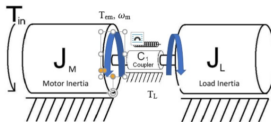
Fig.5. Mechanical system showing Torque, Moment of Inertia and Angular velocity
