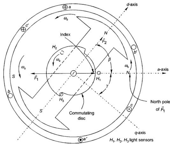
Fig.4. Rotor Position illustrations
