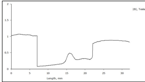
Fig.1. Plot of magnetic field intensity vs length of selected line
