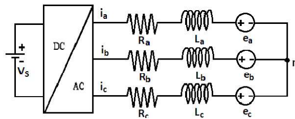
Fig.3. Equivalent circuit of three phase star connected inverter
