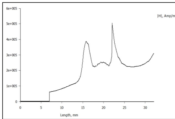
Fig.2. Plot of magnetic field density vs length of selected line
